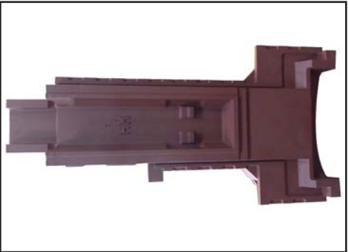
Tailor Made VMC Column For Europe Client
