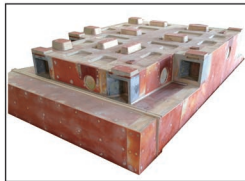
Wooden Pattern With PVC Coated
