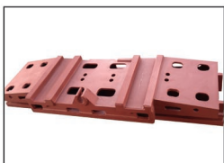
VMC Saddle
